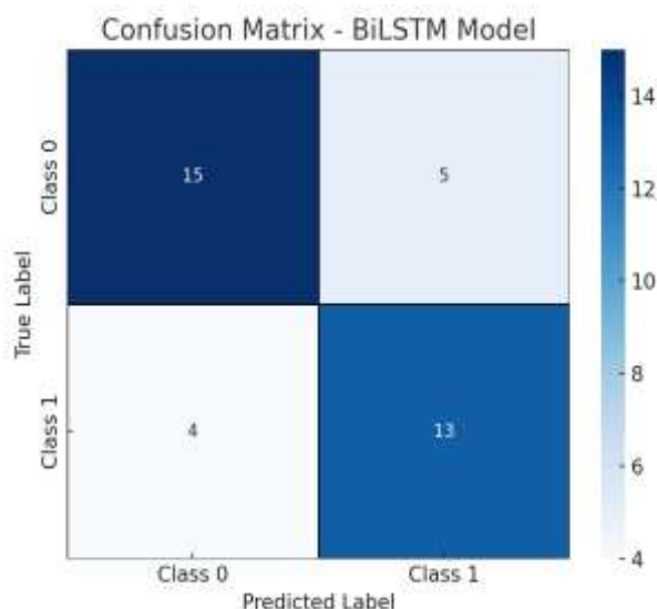
Figure 4: Confusion matrix using BiLSTM
