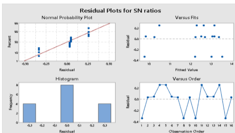
Figure 5.1.2.2: Residual Plots for SN ratios for Flexural Strength (M40)
