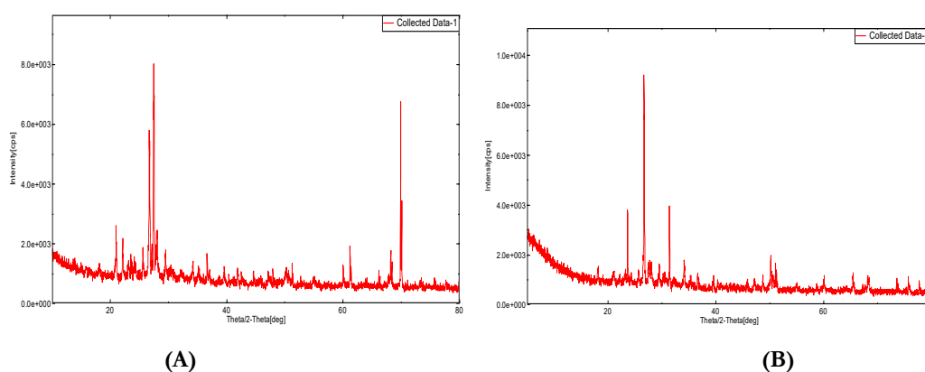
Figure 5.1.4: XRD of M40 Controlled Mix (A) & M40 L4 Mix (B) Cured for 90Days
