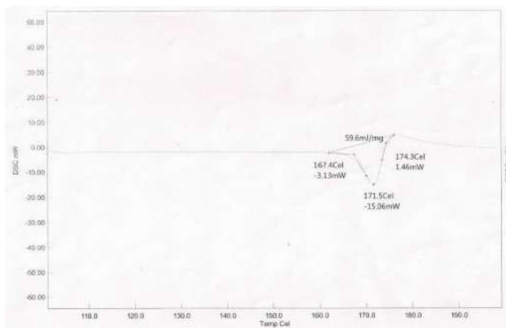
Figure 5a. DSC thermogram of telmisartan cilexetil with excipients at day zero, showing endothermic melting onset at 167.4°C and peak at 171.5°C ( \Delta H = 59.6 mJ/mg).
