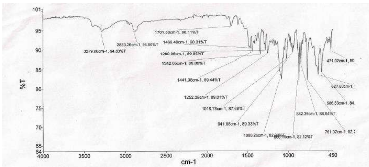
Figure 2b: FTIR spectrum of asenapine maleate with all excipients after 1 month at 40°C/75% RH. Preservation of all characteristic peaks and absence of new bands confirm physicochemical compatibility.
