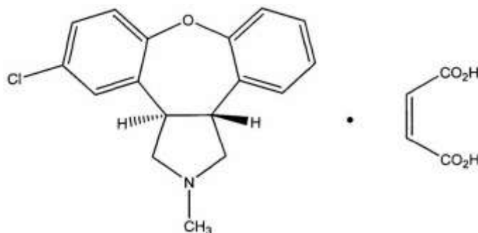
Figure 1: Chemical structure of asenapine maleate ( \text{C}_{21}\text{H}_{20}\text{ClN} \cdot \text{C}_4\text{H}_4\text{O}_4 ; MW 401.84 g/mol), showing the tetracyclic dibenzoxepine core and the maleic acid counterion essential for salt stability.
