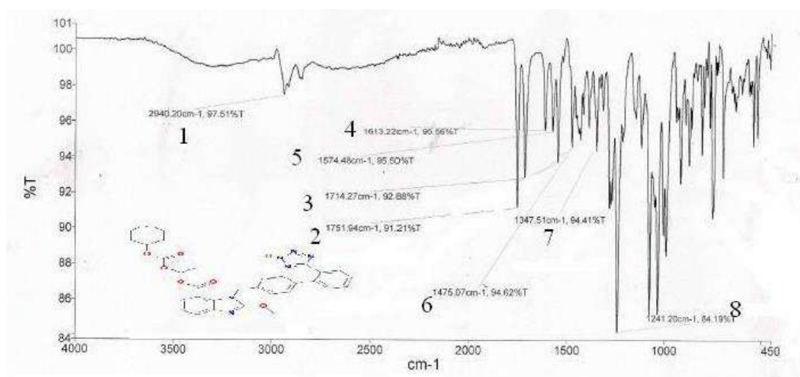
Fig. 4b. FTIR spectrum of telmisartan cilexetil with all excipients after 1 month at 40°C/75% RH. Preservation of all characteristic absorption bands confirms physicochemical compatibility of TC with the intended excipient blend.
