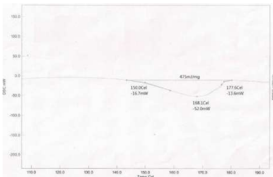
Figure 5b. DSC thermogram of telmisartan cilexetil with excipients after 1 month at 40°C/75% RH. Broadened endotherm with onset at 150°C and peak at 168.1°C reflects minor polymorphic transitions under stress, without evidence of chemical degradation.
