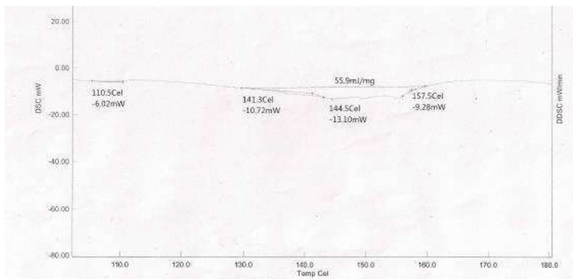
Figure 3a: DSC thermogram of asenapine maleate with excipients at day zero showing endothermic melting onset at 141.3°C, consistent with the pure drug reference.
