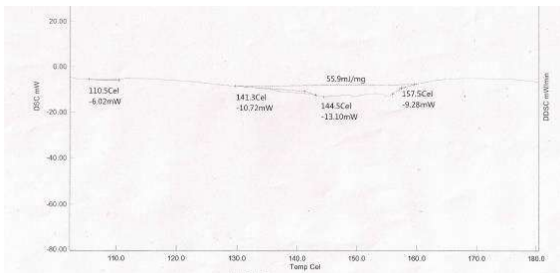
Figure 3b: DSC thermogram of asenapine maleate with excipients after 1 month at 40°C/75% RH. Unchanged melting onset confirms no drug-excipient incompatibility.
