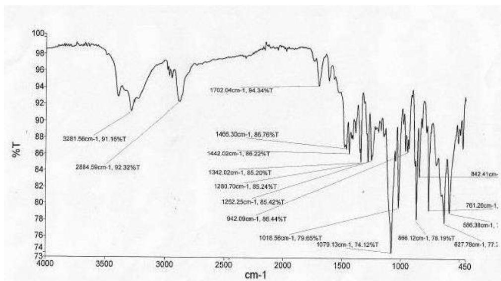
Figure 2a: FTIR spectrum of asenapine maleate pure drug (day zero, room temperature) showing characteristic functional group absorption bands. Key assignments: 2884 cm -1 (N-CH 3 stretch); 1702 cm -1 (C=O carboxylate, maleate); 1466/1442 cm -1 (aromatic C=C); 1342 cm -1 (C–O–C bend).
