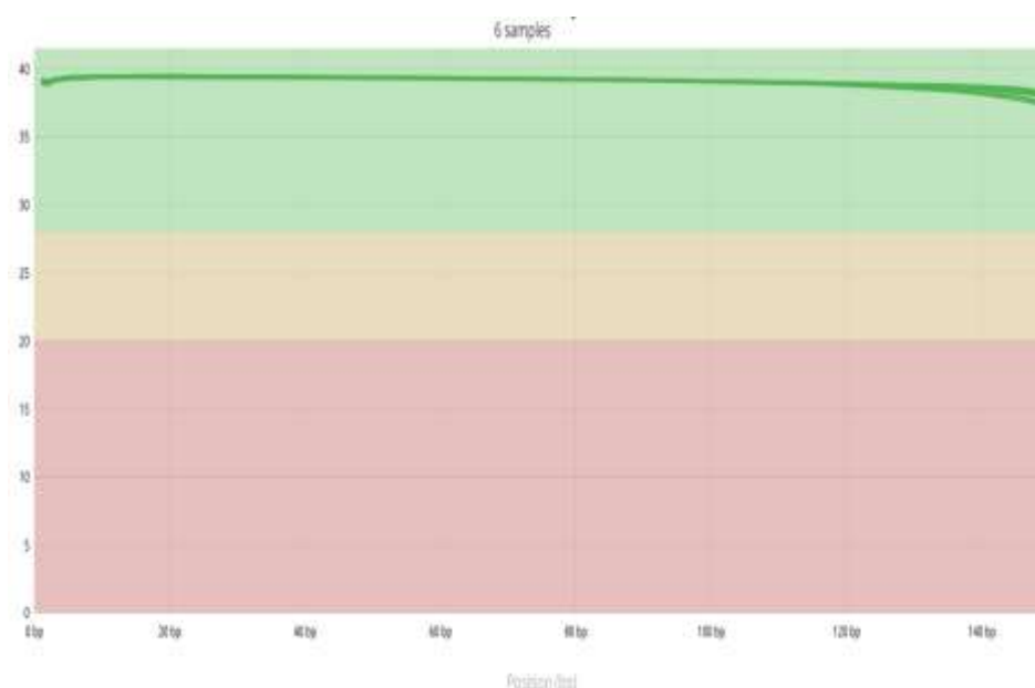
Figure 2. Per-base sequence quality of raw sequencing reads for Phage-1 (1A), Phage-2 (2A) and Phage-3 (3A) (MultiQC/FastQC).
