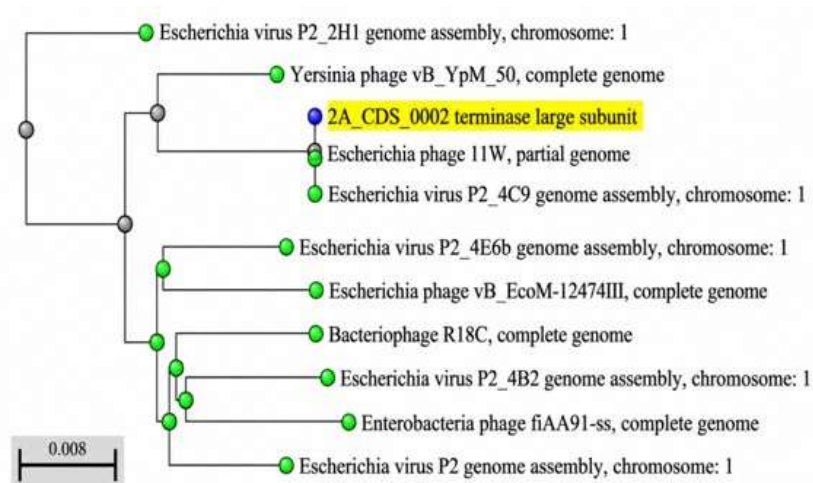
Figure 7. Terminase large-subunit (terL)-based phylogenetic tree of Phage-2 (2A) and related phage sequences.
