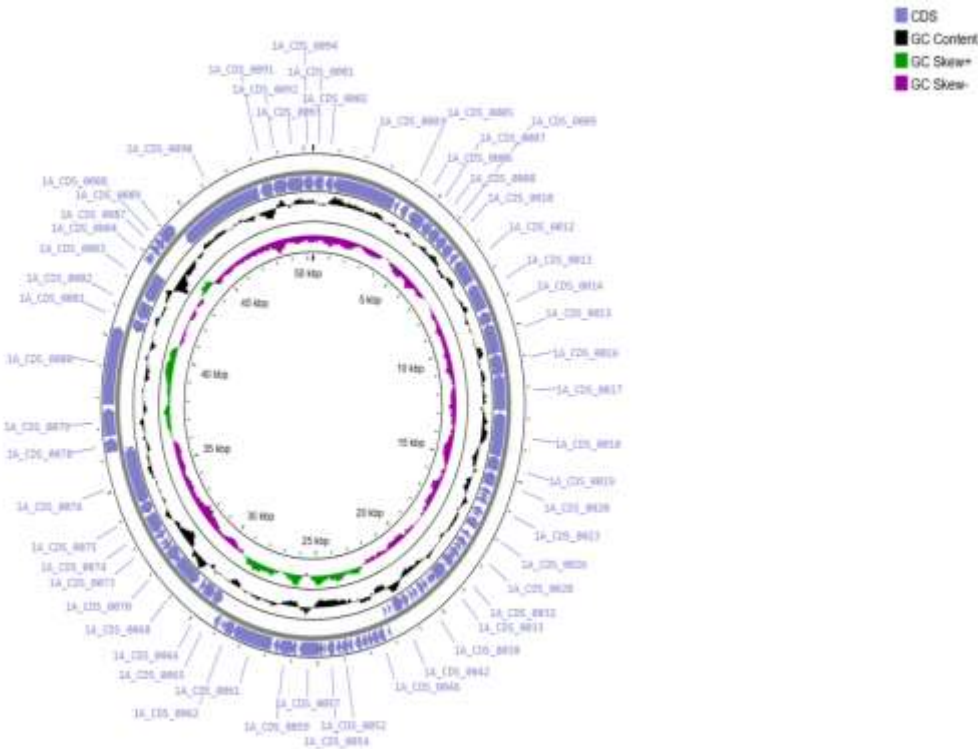
Figure 3. Circular genome map of Phage-1 (sample 1A), showing the organization of predicted genomic features across the 50,343-bp assembled genome
