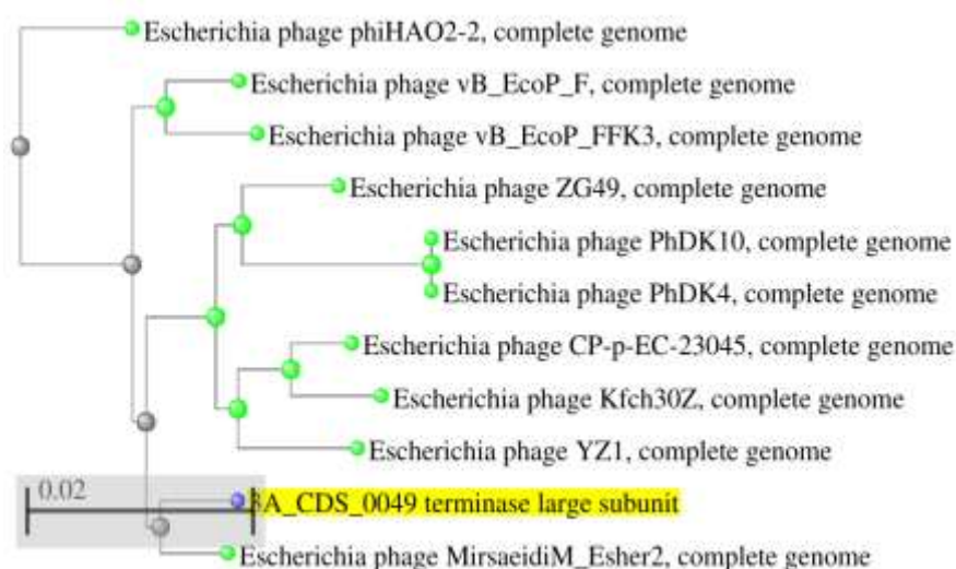
Figure 8. Terminase large-subunit (terL)-based phylogenetic tree of Phage-3 (3A) and related phage sequences.
