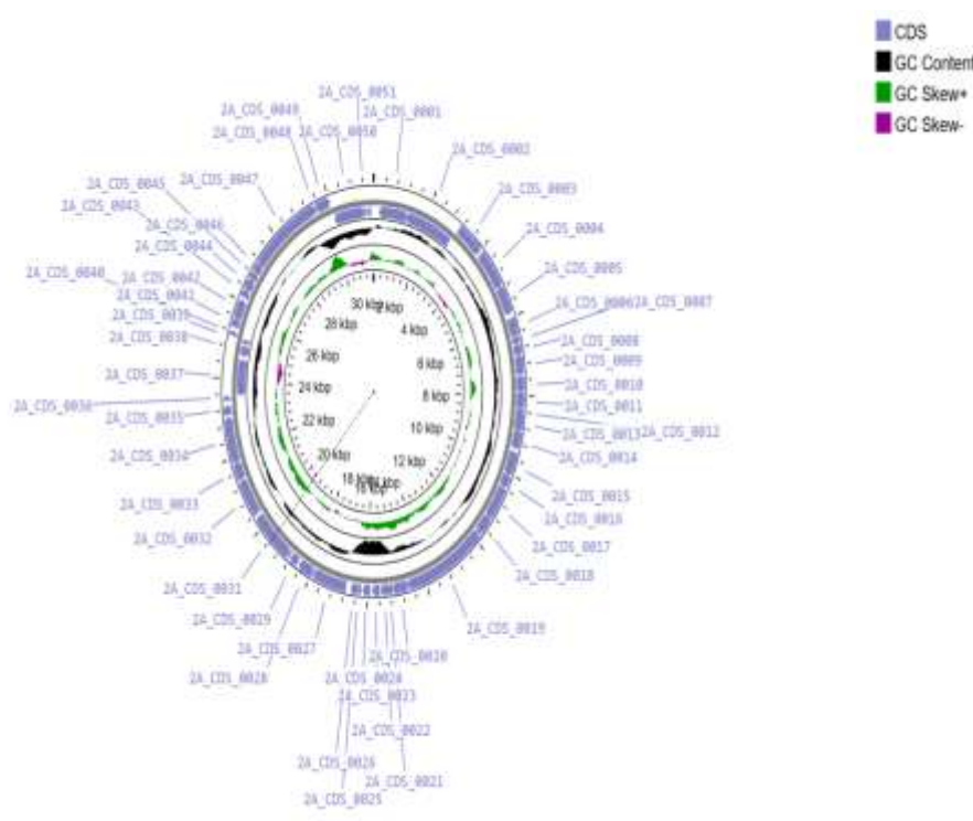
Figure 4. Circular genome map of Phage-2 (sample 2A), showing the organization of predicted genomic features across the 31,564-bp assembled genome.
