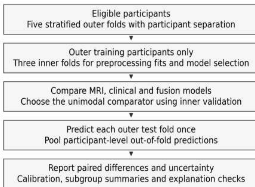
Figure 2. Proposed validation and reporting workflow. All fitted clinical transformations, tuning and comparator selection occur within the outer training participants.
